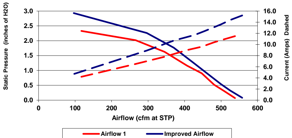
Example of Airflow Performance
